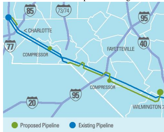
Figure B. Piedmont Natural Gas Pipeline Serving Sutton Power Plant 8
